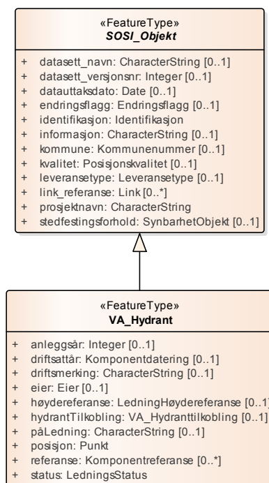
Figur 29: Hoveddiagram: VA_Hydrant
