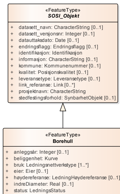
Figur 1: Hoveddiagram: Borehull
